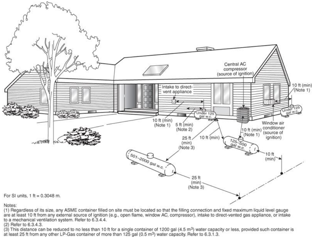
FIGURE I.1 (b) Aboveground ASME Containers. (This figure for illustration purposes only; written code shall govern)
